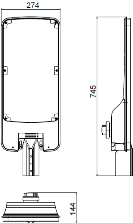
1-10V + NEMA Socket Version
