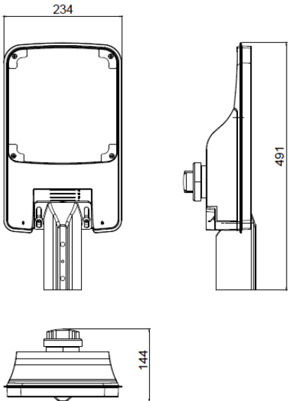
1-10V + NEMA Socket Version
