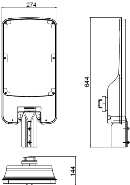
1-10V + NEMA Socket Version
