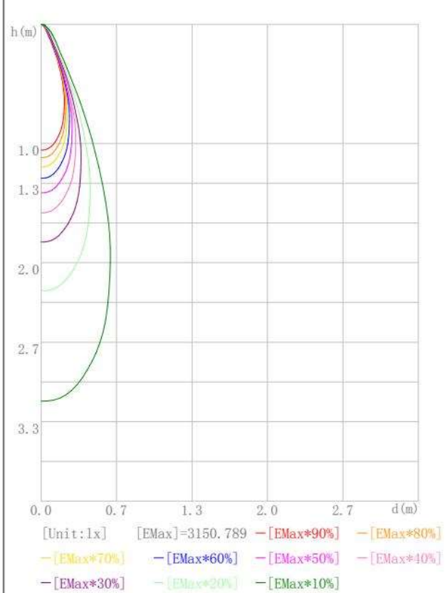
C0 Space ISO Illuminance Curve
